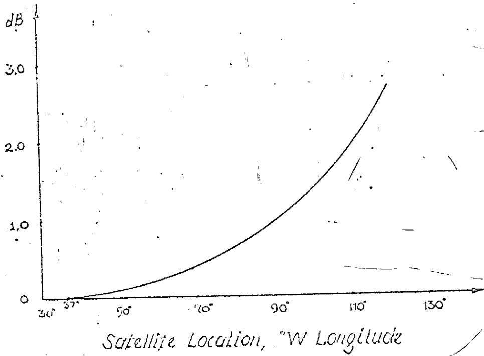
Figure IV - Additional Losses VS. Satellite Location
